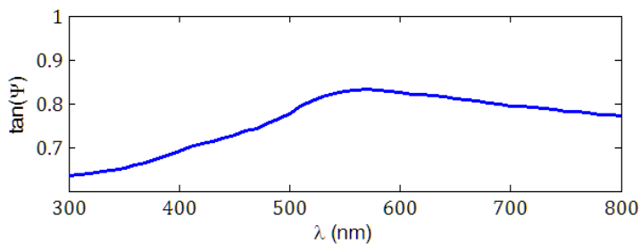
Figure 3 - Trajectories of tg(\psi) for gold 585 strip, annealed, specimen (1);
