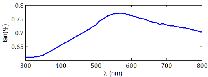
Figure 4 - Trajectories of tg(\psi) for gold 585 strip, a0% deformation, specimen (2)
