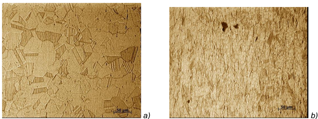
Figure 7 - Microstructure of gold 585 strip: a) annealed at 680°C and b) cold deformed 30%
