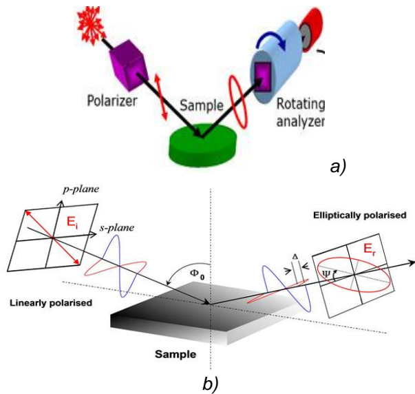
Figure 1 - From known input of linearly polarized beam a) and definitions \psi and \Delta for measuring at reflected elliptically polarized beam b)
