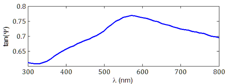
Figure 6 - Trajectories of tg(\psi) for gold 585 strip, 30% deformation, specimen (4)
