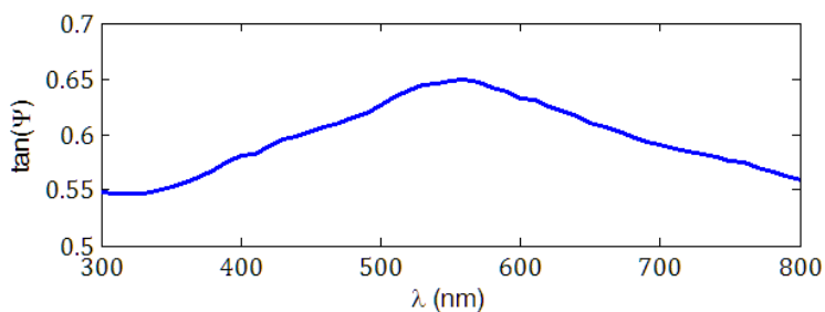
Figure 5 - Trajectories of tg(\psi) for gold 585 strip, 20% deformation, specimen (3)
