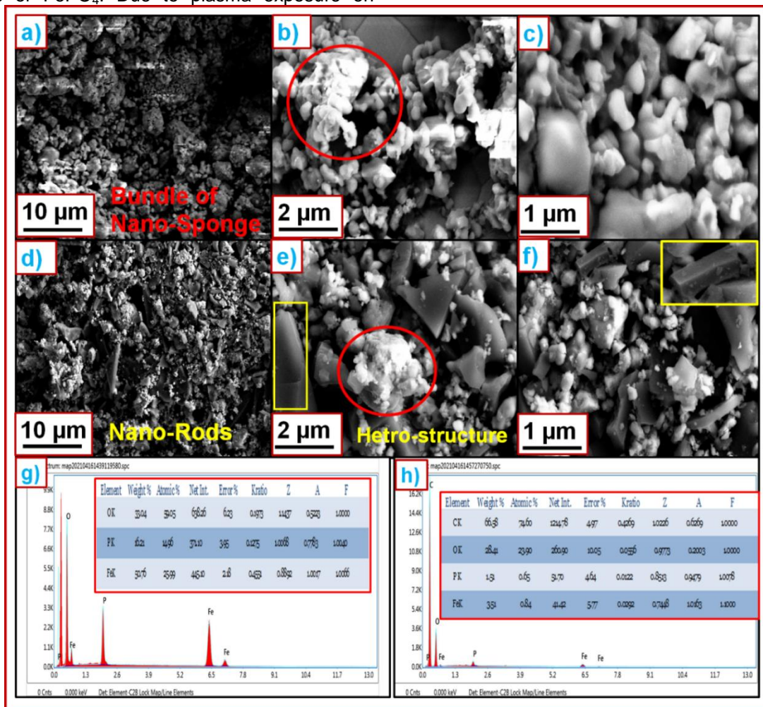
Figure 3. FESEM analysis of pure FePO 4 and FePO 4 /plasma exposed BCC (a-c) Bundle of pure FePO 4 (d-f) Hetero structure of bundle of nano sponge and nano rods of FePO 4 /plasma exposed BCC (g) EDAX spectrum of Pure FePO 4 (h) EDAX spectrum of FePO 4 /plasma exposed BCC
