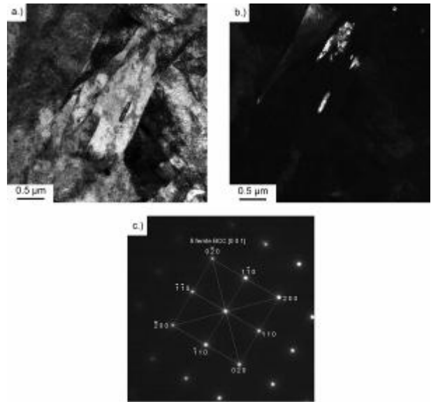
Figure 6 - TEM images of \alpha' -ferrite phase in sample 1: (a) bright field image; (b) dark field image; (c) corresponding selected area diffraction pattern
