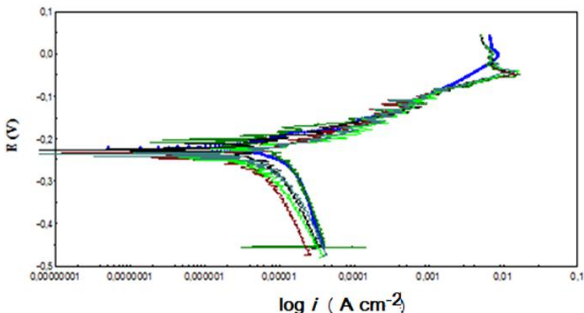
Figure 2. Anodic and cathodic polarization curves of bronze in 3% NaCl with and without the addition of Polka Maglaj leaf extract at different concentrations: ---3% NaCl; ---3% NaCl+0.01612 \text{gdm}^{-3} ; ---3% NaCl+0.03221 \text{gdm}^{-3} ; ---3% NaCl+0.04828 \text{gdm}^{-3} ; ---3% NaCl+0.06432 \text{gdm}^{-3} ; ---3% NaCl+0.08033 \text{gdm}^{-3}
