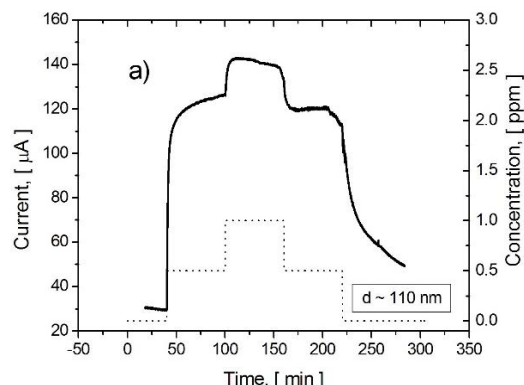
Figure 12. Transient characteristics of gas - induced current by exposure of Te films (thickness \sim 110 nm) to various concentrations of \text{NO}_2 according to the profile shown in dotted lines of the bottom. Substrate: Pyrex – glass
