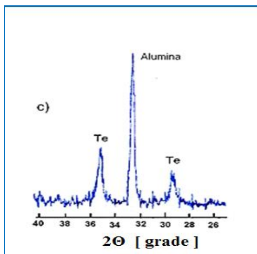
Figure 8. XRD diffraction micrographs of Te get o Al 2 O 3 substrate with deposition rate v = 30 \text{ nm/s}
