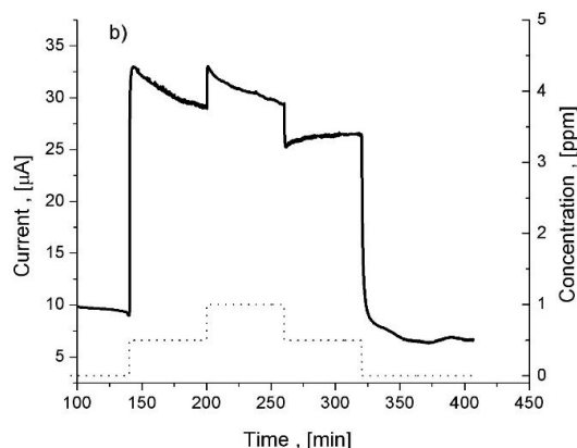
Figure 13. Transient characteristics of gas - induced current by exposure of Te films (thickness \sim 110 nm) to various concentrations of \text{NO}_2 according to the profile shown in dotted lines of the bottom. Substrate: Nanostructured \text{Al}_2\text{O}_3
