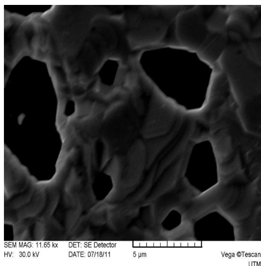
Figure 7. SEM micrographs of Te film deposited on Al 2 O 3 substrate with deposition rate v = 30 \text{ nm/s}
