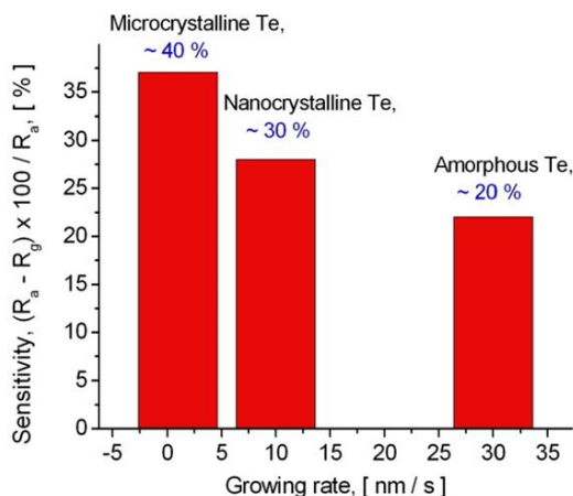
Figure 11. The sensitivity of Te thin films to 1 ppm of \text{NO}_2
