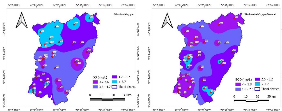
Figure 6. Spatial distribution of a) DO b) BOD
