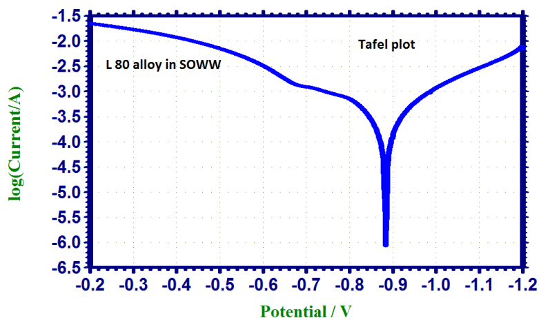
Figure 1. Polarisacion curve of L 80 alloy immersed in SOWW
