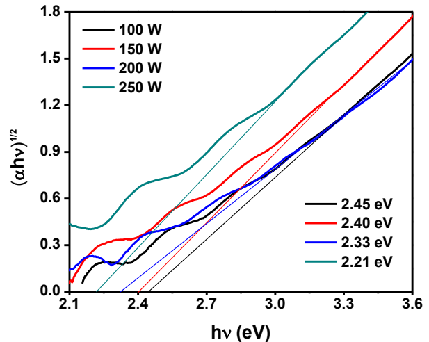
Figure 5. (ah\nu)^{1/2} versus (h\nu) plot of a-SiC thin films deposited on glass substrate at various sputtering pressure
