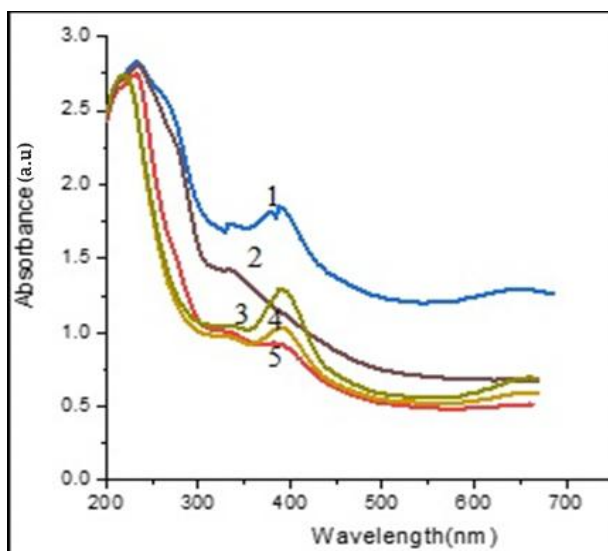
Figure 1. UV absorption spectra 1: \text{Ni}^{2+} +TSC+Gly+ c-BN, 2) Nano c-BN, 3) \text{Ni}^{2+} +c-BN, 4) \text{Ni}^{2+} +Gly+ c-BN, 5) \text{Ni}^{2+} +TSC+ c-BN
